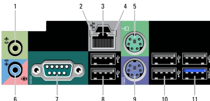
Figur 2. Bakpanelsvy
